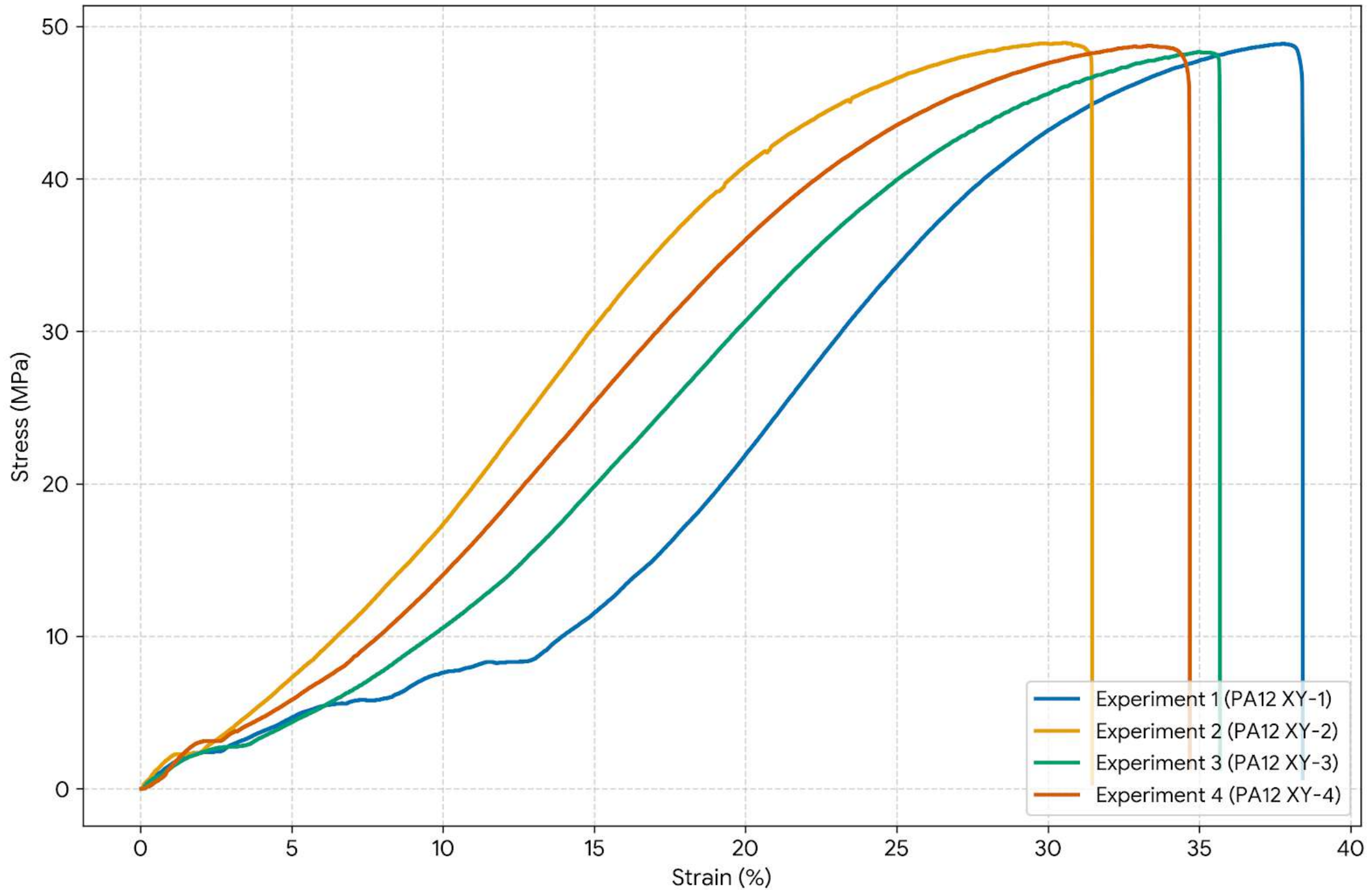
Stress-Strain Curves for PA12 XY (4 Experiments)
